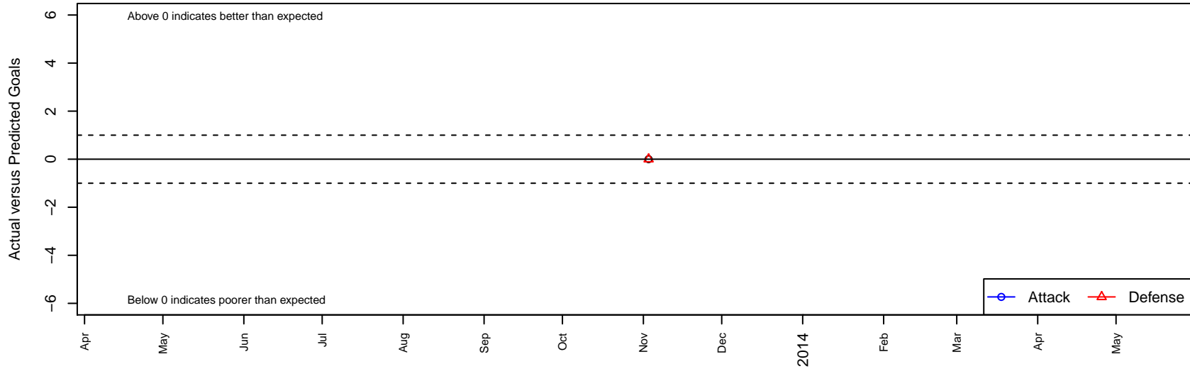
Arsenal FC South B96 Dots are actual minus expected GF (blue circles) and GA (red triangles). Blue line is smoothed change in attack strength. Red is smoothed change in defense strength.
